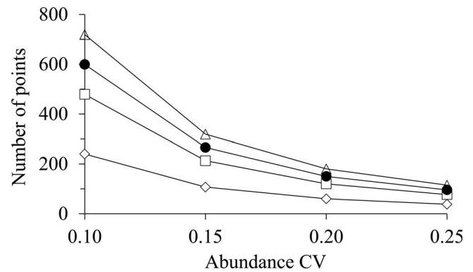
FIGURE 4. Number of survey points needed for abundance CV = 0.10–0.25, when the Grenada Dove spatial distribution is random (diamonds: dispersion parameter [ b ] = 1) or clumped (squares: b = 2 ; triangles: b = 3 ). For survey planning, we assumed that spatial distribution was clumped (circles: b = 2.5 ).
