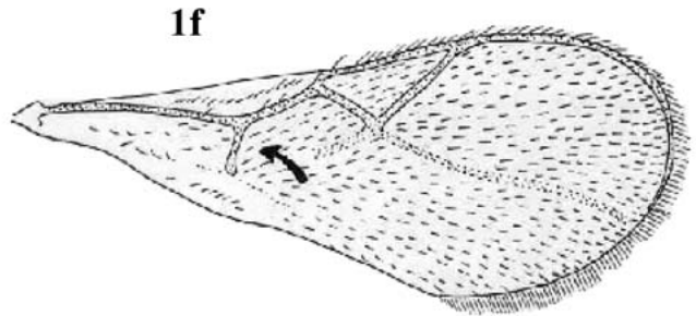
Fig. 1. Aganaspis alujai . a, female antenna; b, pronotal plate; c, scutellar disc and cup in profile; d, scutellar disc and cup in dorsal view; e, fore, mid, and hind coxae in lateral view; f, complete fore wing, with arrow showing the area behind Rs&M vein between Sc+R1 and basal section of Cu1.
