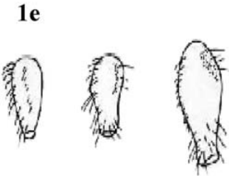
Fig. 1. Aganaspis alujai . a, female antenna; b, pronotal plate; c, scutellar disc and cup in profile; d, scutellar disc and cup in dorsal view; e, fore, mid, and hind coxae in lateral view; f, complete fore wing, with arrow showing the area behind Rs&M vein between Sc+R1 and basal section of Cu1.
