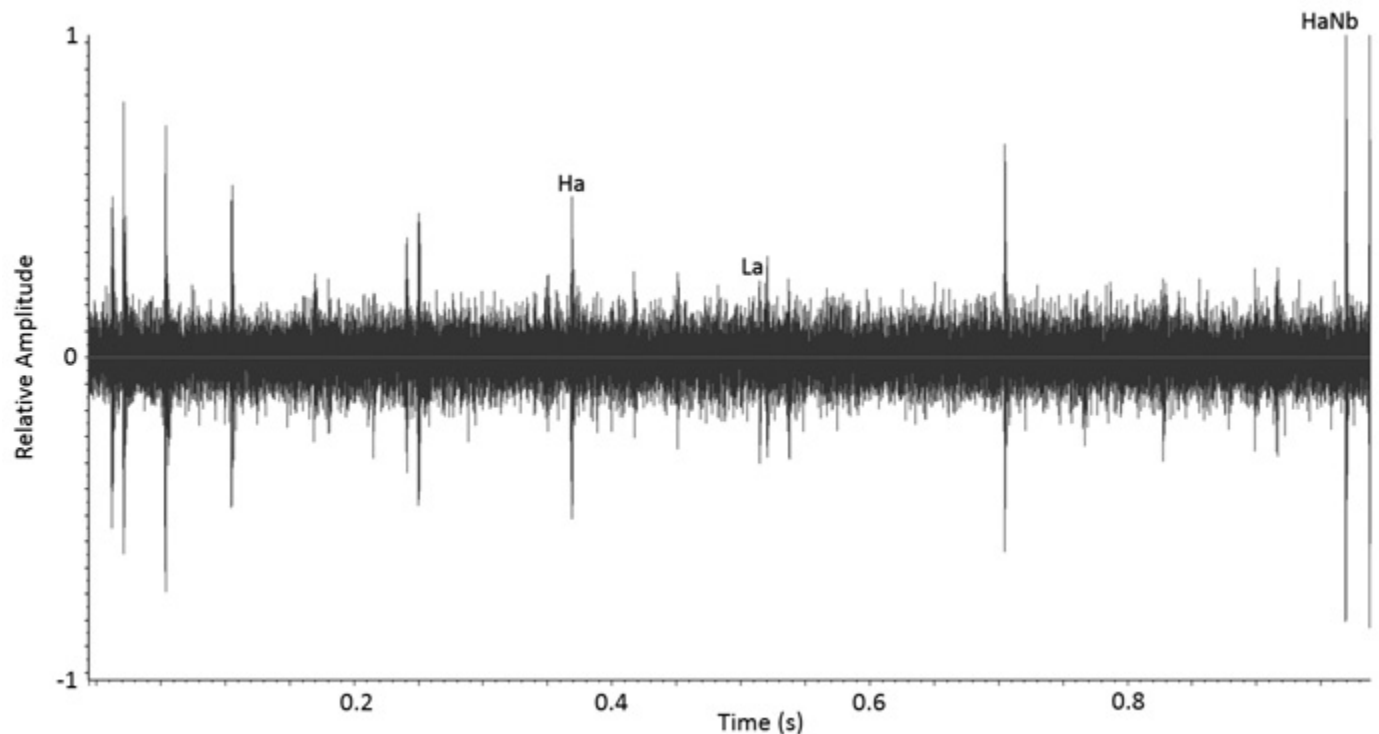
Fig. 2. Oscillogram of sound impulses recorded 10 cm from pouch containing Sitophilus oryzae larvae. Examples of 3 types of larval sound impulse occur during the 1 s period, and one example each of type (Ha, La, and HaNb) is marked above the impulse. Horizontal axis indicates time in seconds and vertical axis indicates relative signal amplitude.
