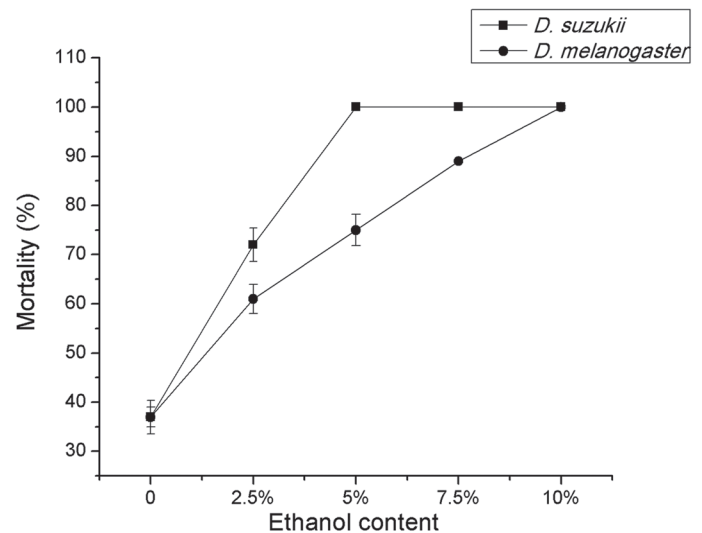
Fig. 3. Mortality of Drosophila melanogaster and Drosophila suzukii larvae exposed to varying concentrations of ethanol.
