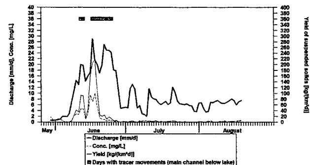
FIGURE 5. Daily specific runoffs, concentrations, and yields of suspended sediments; Outlet Latnjavagge, outlet lake and inlet lake Latnjajaure: (a) 2000 field season, (b) 2001 field season.
