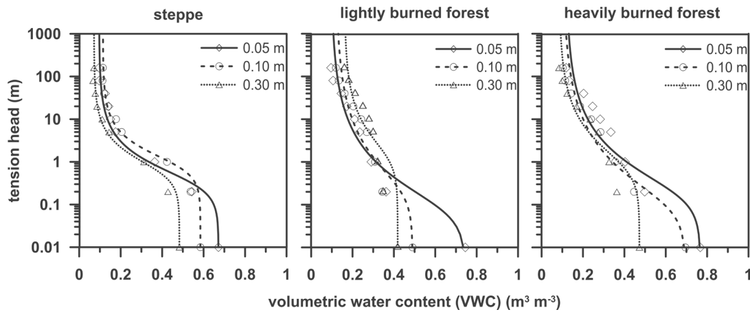
FIGURE 8. Results of the variation in soil moisture content determined from the pressure plate analysis of the soils from the steppe, lightly and heavily burned forest slopes, each at a depth of 0.05, 0.1, and 0.3 m. The best-fit curves were defined according to the method proposed by van Genuchten (1980).
