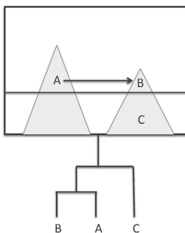
FIGURE 6. (a) Expected phylogenetic relationship for an adaptive radiation origin of a summit speciation event. (b) Expected phylogenetic relationship for a geographic speciation (vicariant) origin of a summit speciation event.
