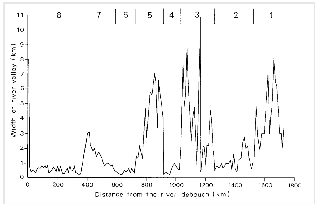
FIGURE 6 Changes in river valley width along the Yaluzangbu main course (based on the Chinese Military Ordnance Map).
