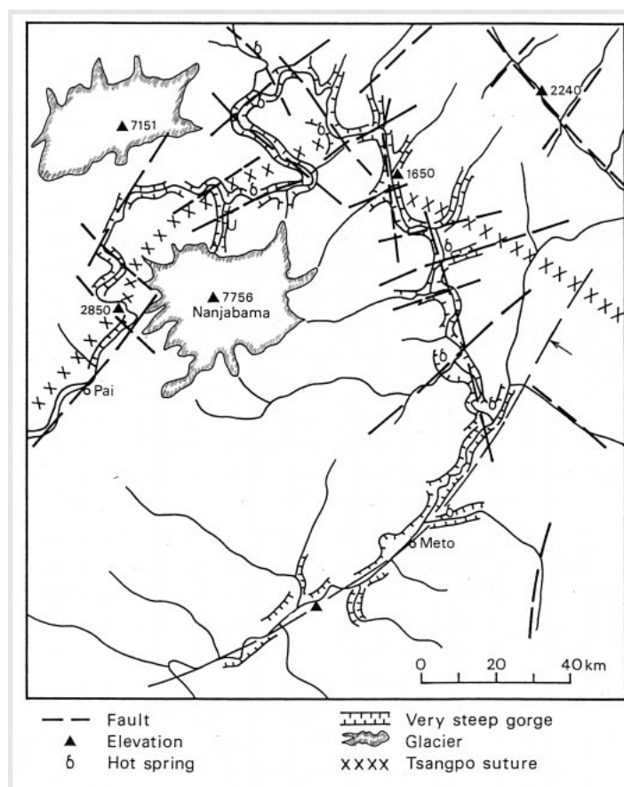
FIGURE 3 Tectonic structures and river channel direction in the Great Bend area (fault source from TETCAS 1983; Zhou et al 1984).
