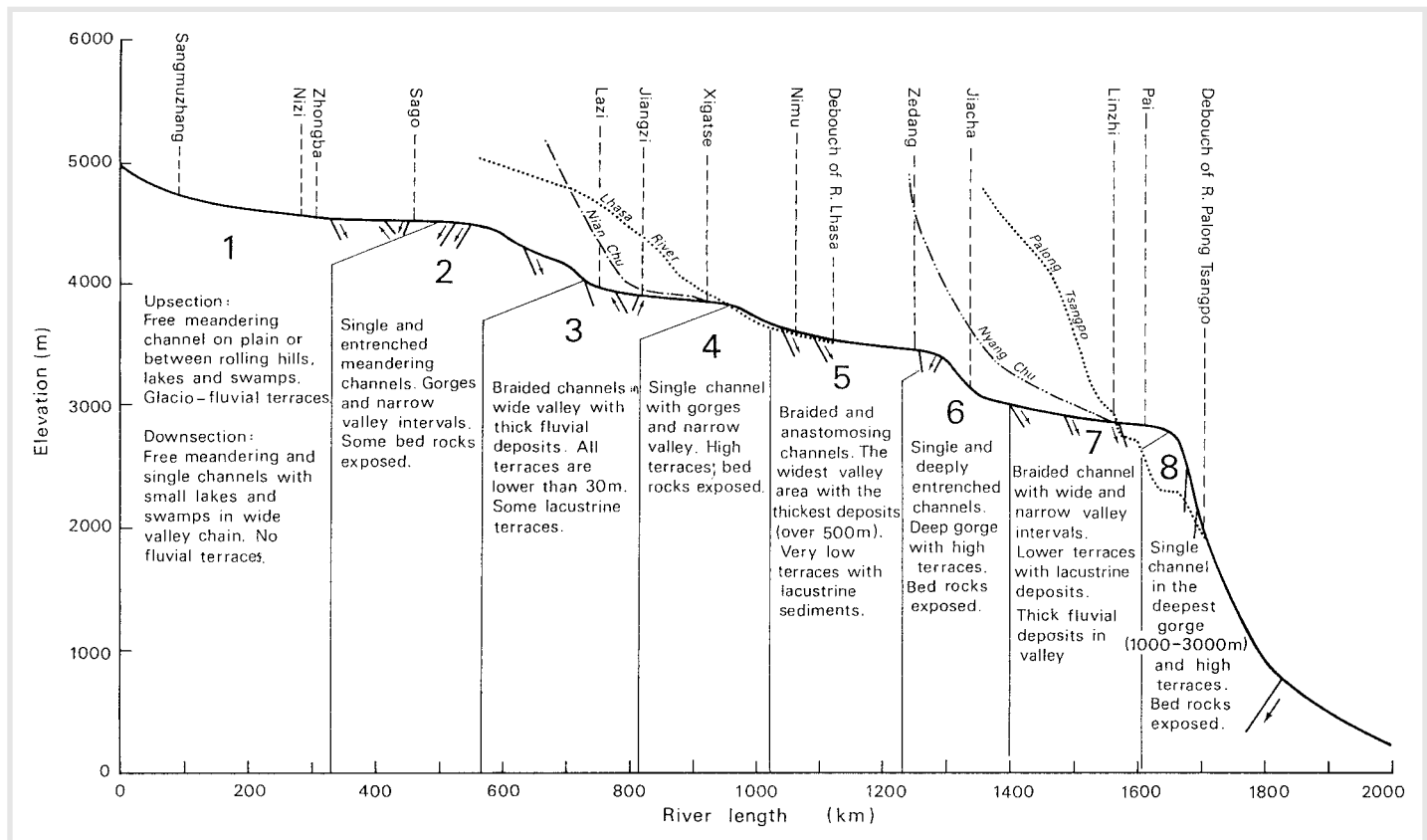
FIGURE 4 Longitudinal profile and the river sections with related fluvial landforms of the Yaluzangbu River (Zhang 1998).
