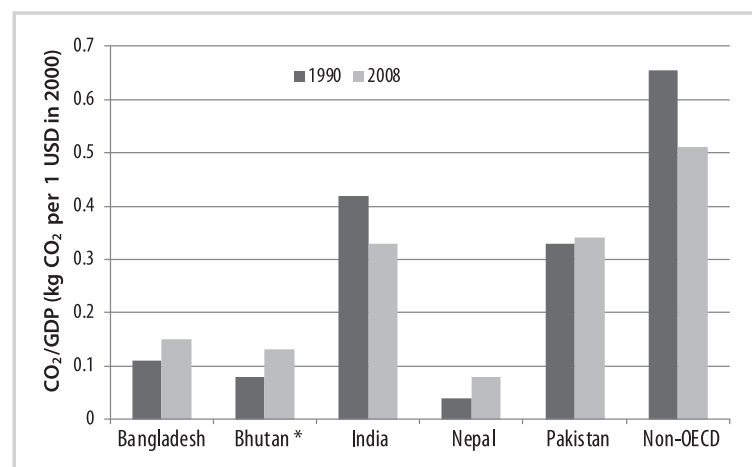
FIGURE 3 CO 2 intensity in 1990 and 2008. Sources: IEA (2010a, 2010b); NEC (2000); UNDP (2007). *Data for Bhutan are from 1994 and 2005.
