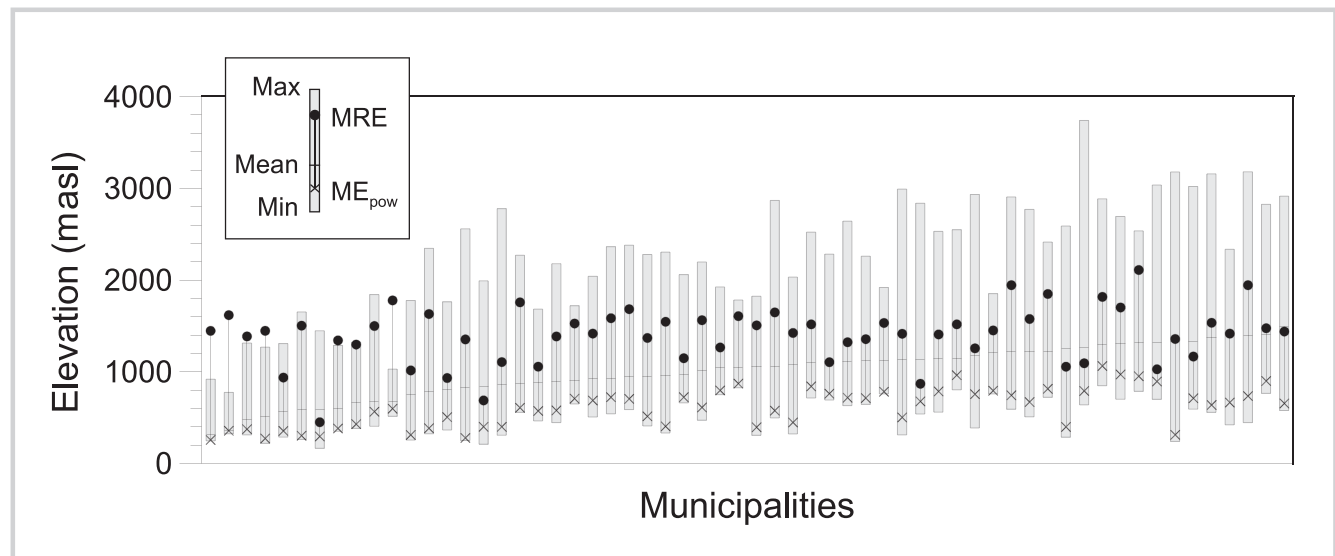
FIGURE 5 Maximum, minimum, and mean elevations of each municipality, with MRE and ME pow . The length of the vertical line connecting MRE and ME pow equals the RPD. Municipalities are ordered by ascending mean elevation.
