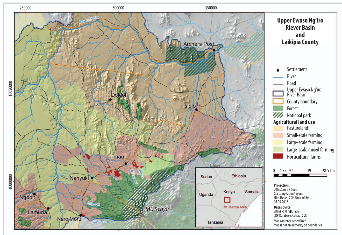
FIGURE 1 Land use including commercial horticulture in the Upper Ewaso North River Basin, 2013. (Data source: this survey, Shuttle Radar Topography Mission v5.0 Hillshade, Laikipai Research Project Database, Centre for Training and Research in Arid and Semi-arid Lands Development (CETRAD) and Centre for Development and Environment (CDE). (Map by Elias Hodel)
