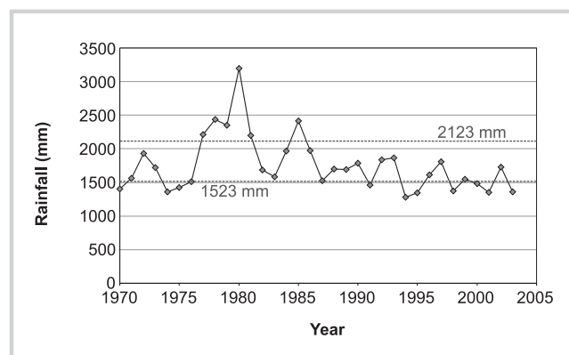
FIGURE 3 Annual rainfall in Finch'a watershed, western Ethiopia. Space between dotted lines indicates the range of assumed normal variation in annual rainfall.
