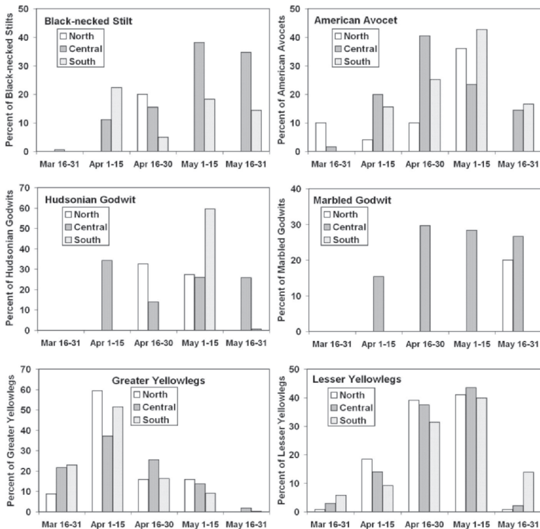
Figure 4. Average (5-year) migration chronology of Black-necked Stilts, American Avocets, Hudsonian and Marbled Godwits, and Greater and Lesser Yellowlegs in the northern, central, and southern regions of Kansas during spring 2002-2006.
