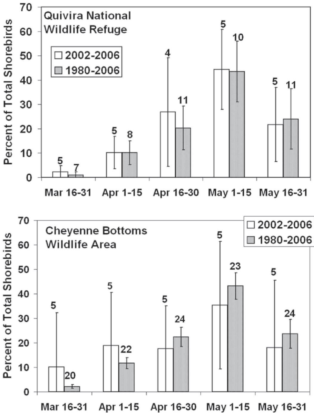
Figure 11. Effect of number of years of surveys on 95% confidence intervals for mean percent of total shorebirds occurring during 2-week periods at Quivira National Wildlife Refuge and Cheyenne Bottoms Wildlife Area. Error bars show 95% confidence intervals. Numbers above error bars are numbers of years of spring surveys.
