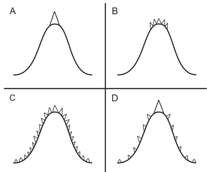
Fig. 4. The four types of Euphasmatodea proventricular dentition. A) A single row of spinules on ridge apex, as in Peruphasma schultei and Aretaon asperimus . B) Many irregularly arranged spinules on the ridge apex, as in Medauroidea extradentata and Sipyloidea sipylos . C) Many tiny spinules all over the ridges and valleys between them, as in Diapherodes gigantea , Eurycantha calcarata , and Extatosoma tigratum . D) Spinules all over ridges and valleys, with a single row of larger spinules on ridge apex, as in Ramulus nematodes . Not to scale.
