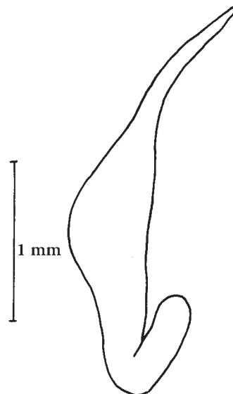
Fig. 7. Titillator of male E. jacquelinae (holotype) in lateral view from right.
