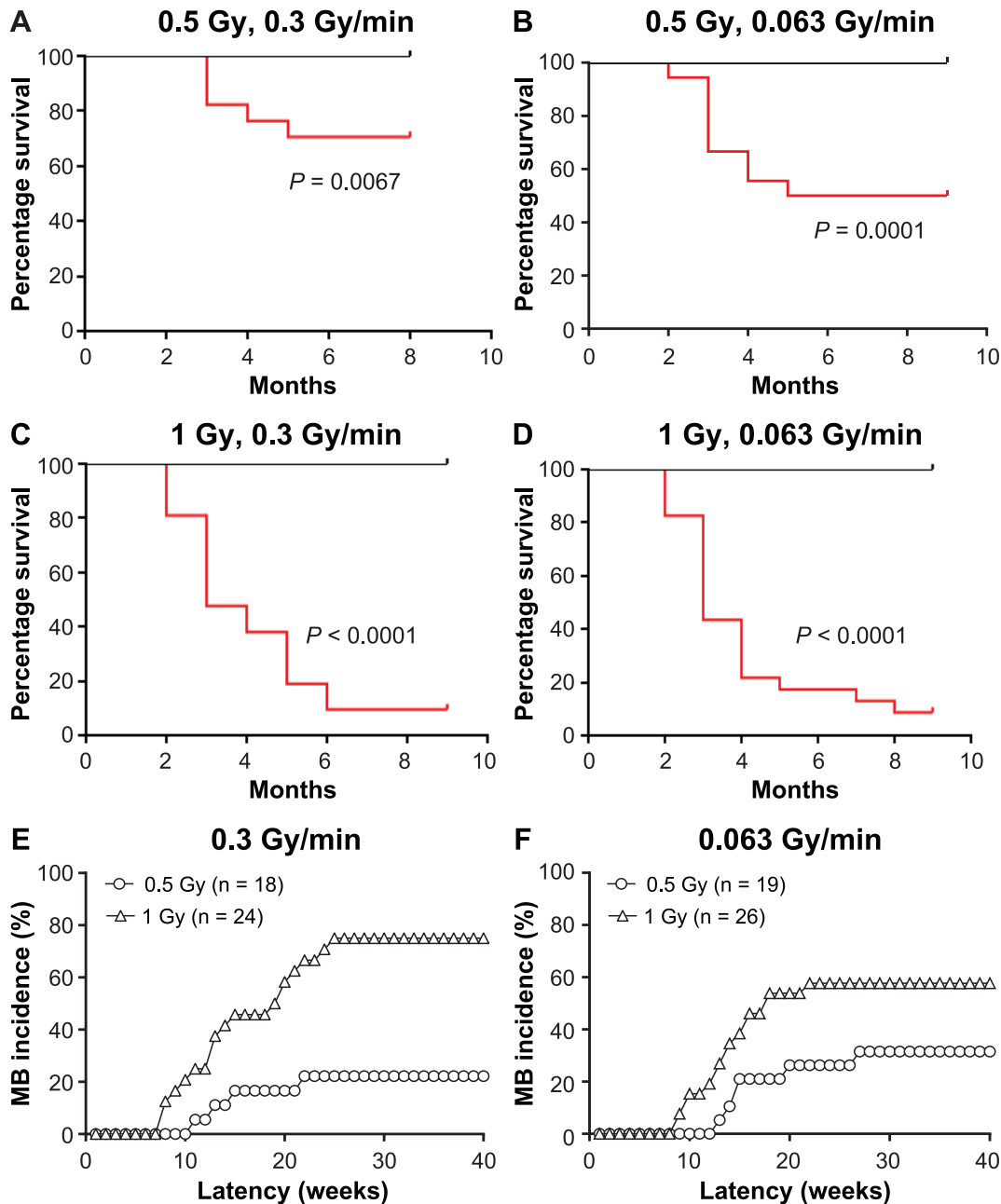
FIG. 3. Dose and dose-rate effects on survival and MB tumorigenesis in Ptch1 +/- /CD1 mice. Mortality of WT and Ptch1 +/- /CD1 mice \gamma -ray irradiated with 0.5 Gy at 0.3 Gy/min (panel A) or 0.063 Gy/min (panel B) or with 1 Gy at 0.3 Gy/min (panel C) or 0.063 Gy/min (panel D). Radiation-induced MB incidences in Ptch1 +/- /CD1 mice irradiated with 0.5 or 1 Gy at 0.3 Gy/min (panel E) or 0.5 or 1 Gy at 0.063 (panel F).
