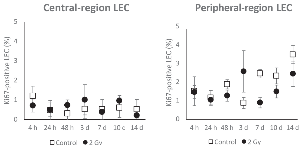
FIG. 3. Percentage of Ki67-positive LEC in the central and peripheral region 4 h to 14 days after 2 Gy X-ray irradiation. SE bars are plotted. Time postirradiation not statistically significant.
