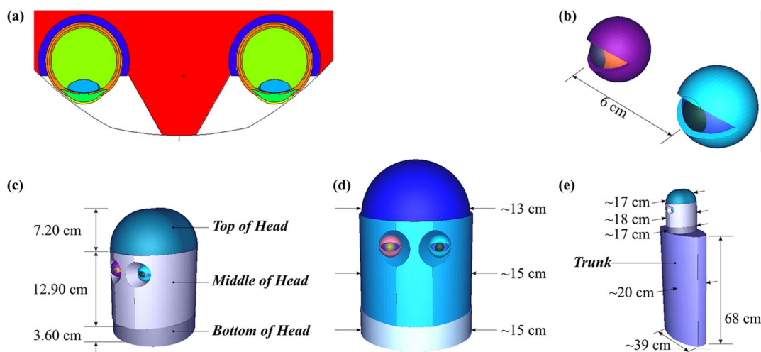
FIG. 2. Views of MTE models embedded in ADAM-EVA phantom generated from MCNP Visual Editor (36). Panel (a): 2D view of multi-tissue eyes coloured by material composition (eye on the right in image is designated as the left eye). Panel (b): 3D view of multi-tissue eyes centered 6 cm apart. Panel (c): 3D view of the three components of phantom head. Panel (d): Head-on 3D view of phantom head. Panel (e): 3D view of overall ADAM-EVA phantom including trunk.
