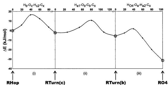
FIG. 5. Energy change upon sequential hydrogen bond rearrangement, relative to RHop ( -2222.004 atomic units). All dihedral angles (in degrees) are referred to distant carbon atoms C_x further on in the crystal lattice. Circles indicate points that were obtained by full optimization (without constraints).
