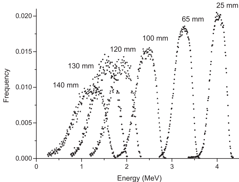
FIG. 4. Spectra of alpha-particle energies incident on the cell monolayer for the specified distances of helium traversed (25–140 mm). The associated mean energy and half-width at half-maximum values are shown in Table 1.
