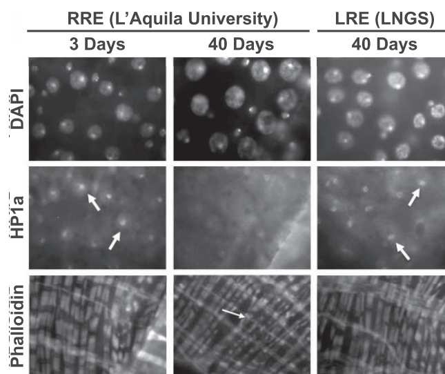
FIG. 3. Age-dependent loss of heterochromatin is prevented by low-radiation environment (LRE). Gut tissues from young (3-day-old) and old (40-day-old) reference radiation environment (RRE) female flies and from old (40-day-old) low-radiation environment (LRE) female flies were dissected and stained with anti-HP1 to visualize the heterochromatin domains and phalloidin-fluorescein to reveal the longitudinal and circular intestinal body wall muscle fibers. Note the presence of marked HP1-enriched foci in the young RRE gut, which appear more diffuse in the old RRE gut but still prominent in old LRE gut (arrows). The phalloidin staining reveals that muscle fibers in old LRE flies are indistinguishable from that of young RRE flies, whereas, as expected, their morphology appears degenerated in old RRE flies.
