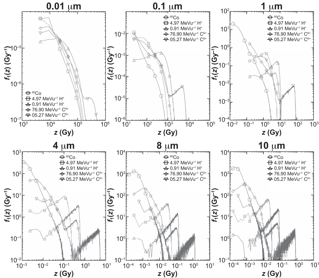
FIG. 2. Frequency distribution of specific energy for one track f_1(z) calculated for spheres with indicated diameters, from 0.01–10.0 \mu\text{m} , for ^{60}\text{Co} , 4.97 \text{MeV u}^{-1} protons, 0.91 \text{MeV u}^{-1} protons, 76.9 \text{MeV u}^{-1} carbon ions and 5.27 \text{MeV u}^{-1} carbon ions.
