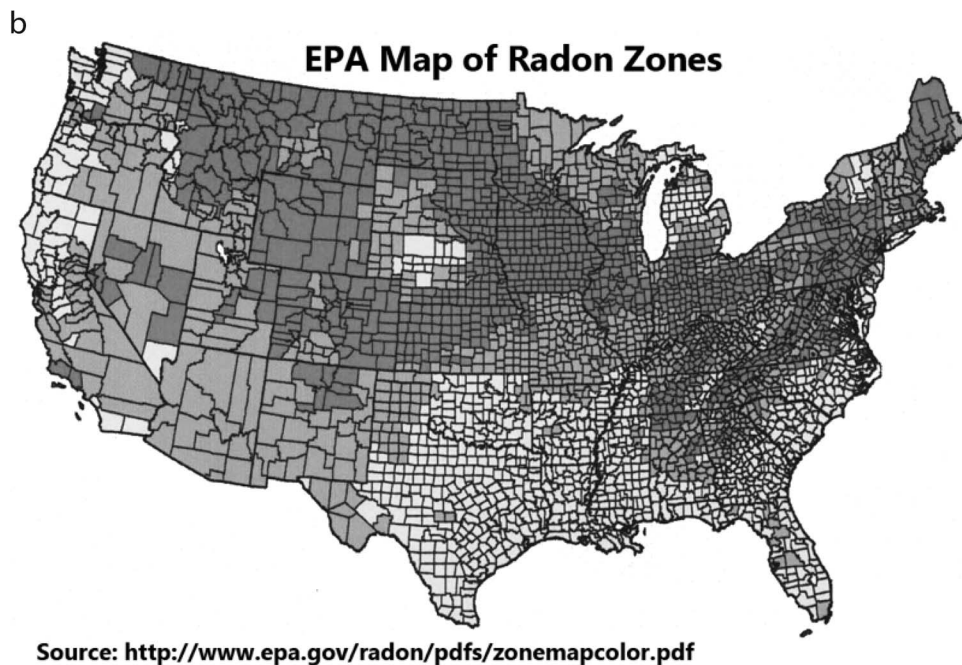
FIG. 1. Panel a: National Cancer Institute map of lung cancer rates in the U.S. 2000–2004. Panel b: Environmental Protection Agency map of radon zones in the U.S.
