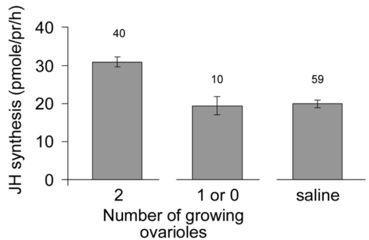
Figure 3. Juvenile hormone (JH) synthesis by the corpora allata of males denervated on day 1, 72 hr after implantation of 2 ovarioles with 1.00mm long basal oocytes. The data in Fig 2B are subdivided into males in which basal oocytes of both ovarioles increased in length (2) and those in which only one or neither increased in length (1 or 0). Controls (saline) for males with denervated corpora allata injected with saline are from Fig 2B. Each column shows the mean \pm SEM of the number of individual measurements above each column.
