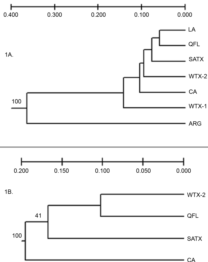
Figure 1. Dendrograms based on Nei's genetic distance (1987) by the method of UPGMA (Sneath and Sokal 1973). Relationships (A) showing the six U.S. geographic populations of Gonatocerus ashmeadi and a population classified as near G. ashmeadi (M2012) from Argentina performed by ISSR-PCR DNA fingerprinting. Field collected populations were also analyzed separately (B). Genetic distances are indicated above the dendrograms and bootstrap support values are indicated at the nodes.
