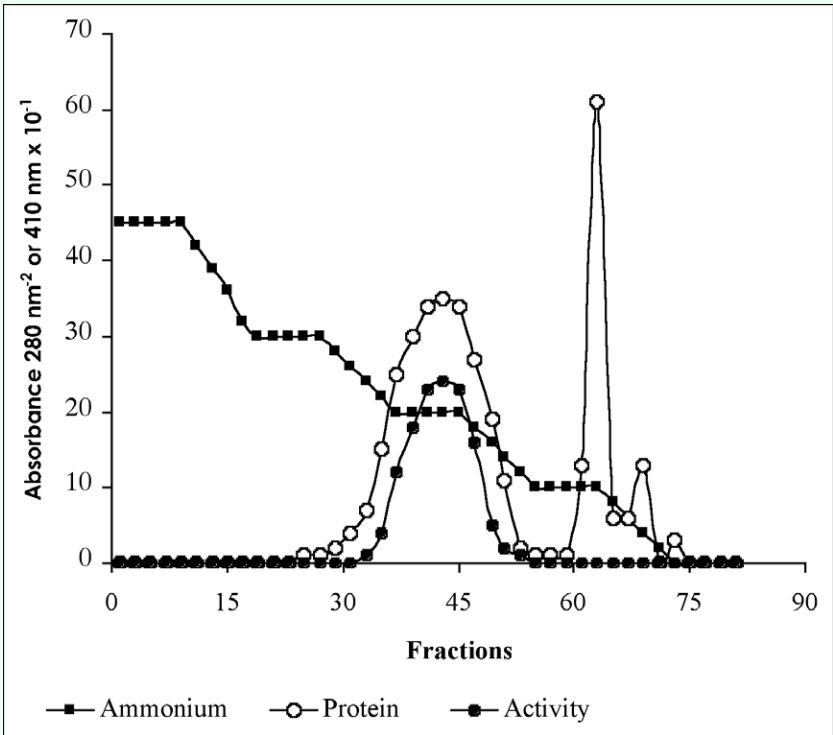
Figure 3. Hydrophobic interaction chromatography of \beta -glucosidase from the digestive juice of the palm weevil Rynchophorus palmarum larvae on Phenyl-Sepharose CL-6B.
