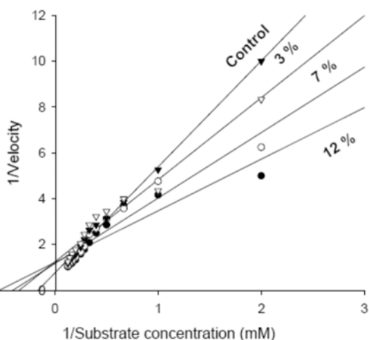
Figure 4. Double reciprocal plot to show the effect of different concentrations of Beauveria bassiana secondary metabolites on the phenoloxidase activity of Eurygaster integriceps adults ( 1/V_{\max} = intercept on the 1/V_0 ordinate, -1/K_m = intercept on the negative side of the 1/(S) abscissa). EtOH was used as control solution. High quality figures are available online.
