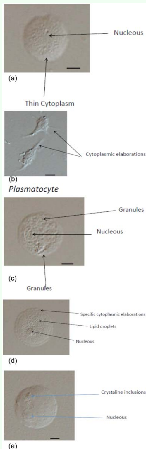
Figure 1. (a-e) Light microscopy of Eurygaster integriceps hemocytes: (a) a prohemocyte with a large nucleus (thin arrow) and a thin cytoplasm; (b) a plasmatocyte exhibiting a spindle shape and cytoplasmic elaborations; (c) a granulocyte filled with the typical granules in the cytoplasm (arrow) and large nucleus (arrow); (d) an adipohemocyte with lipid droplets spreading in the cytoplasm and specific cytoplasm elaborations; (e) an oenocytoid with a round eccentric nucleus and crystalline inclusions. Magnification 40 \times with the exception of (b) (60 \times ). Bar = 5 \mu\text{m} , with the exception of (b) (3 \mu\text{m} ). High quality figures are available online.
