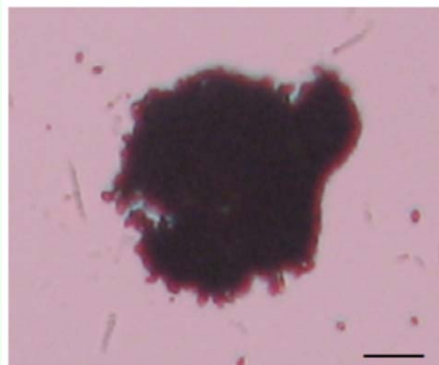
Figure 3. Nodule formation in Eurygaster integriceps adults 12 hours after inoculation by Beauveria bassiana spores. Scale bar 10 \mu m. The magnification of images is 40 \times . High quality figures are available online.
