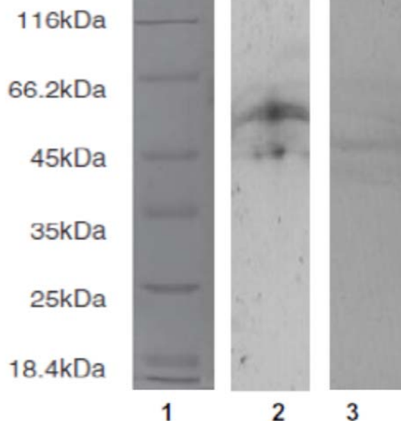
Figure 5. Phenoloxidase isozyme profiles. (1) Molecular marker, (2) control, (3) hemocyte lysate sample after 12-h injection of 15% concentration of secondary metabolite. Samples exposed to Beauveria bassiana secondary metabolite for 12 h versus control. High quality figures are available online.
