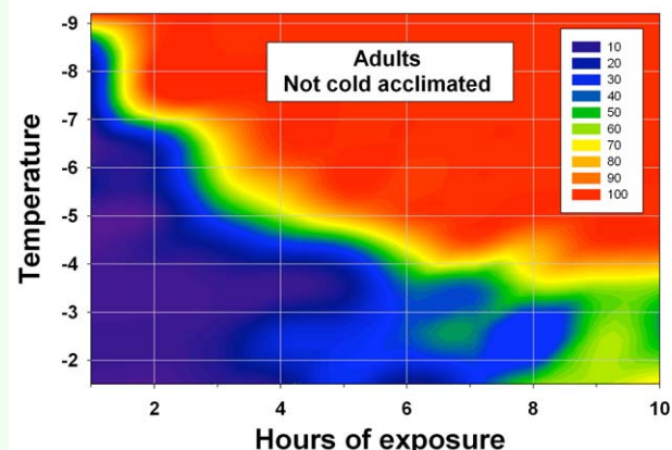
Figure 1. Percent mortality of adult Diaphorina citri after being exposed to from -1.5 to -9.2 ° C for one to ten hours (two replications of five adults of each sex for each temperature/exposure combination, data pooled over both sexes and replications). The adults were from an air-conditioned greenhouse and, thus, not cold acclimated. This figure identifies freeze events that should usually be nonlethal to the adult psyllids irrespective of whether they are cold acclimated. High quality figures are available online.
