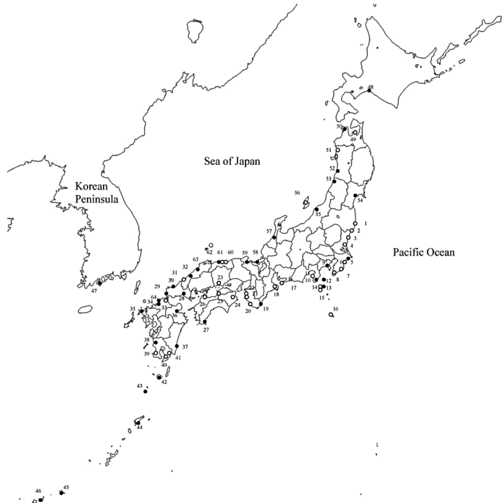
Fig. 1. Sampling localities for S. griseus and S. tigrinus , with population numbers (referenced in Table 1). Closed circles indicate populations included in phylogenetic analysis.
