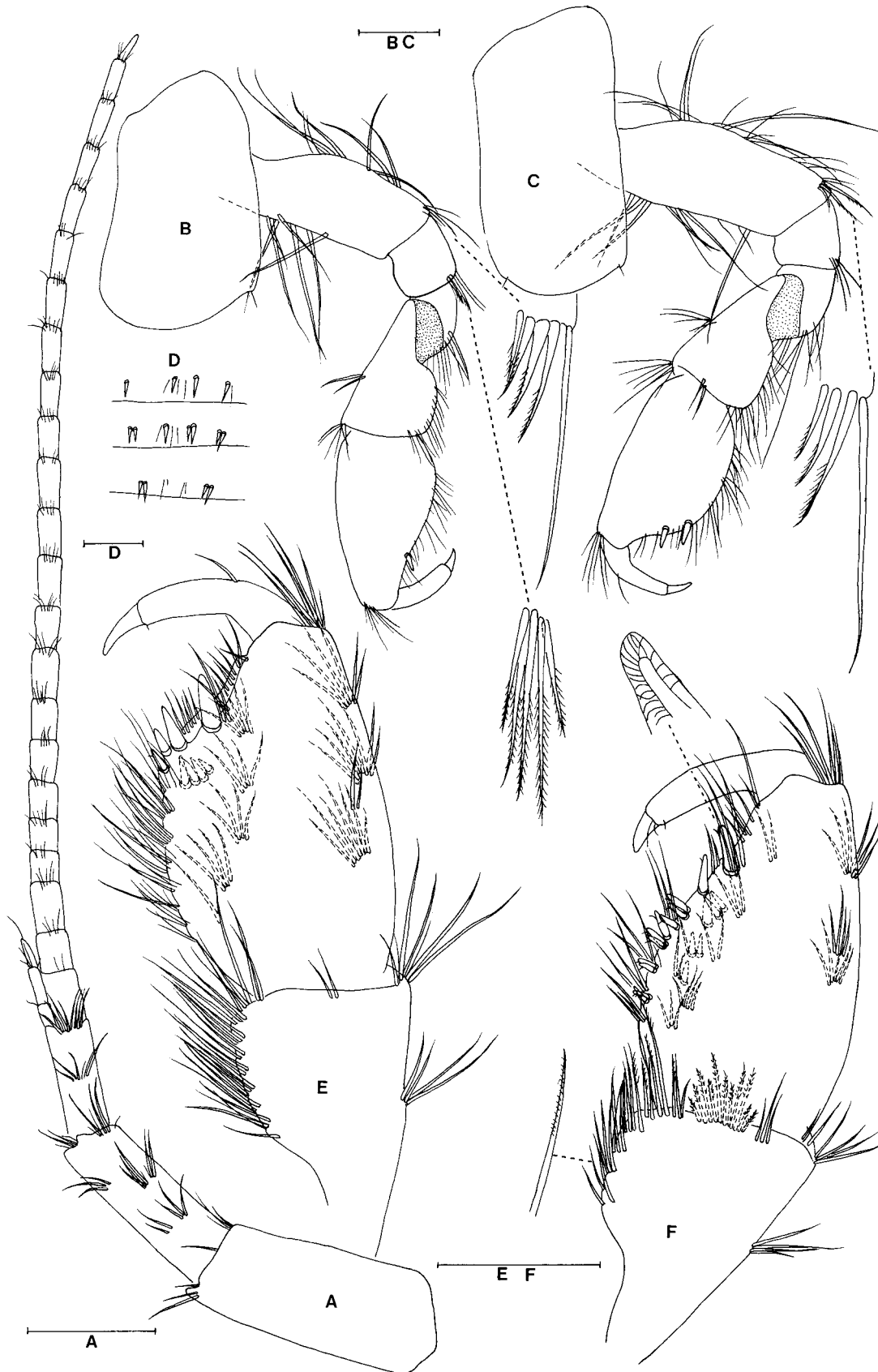
Fig. 8. Gammarus stagnarius sp. nov. holotype, male. A, antenna 1; B, gnathopod 1; C, gnathopod 2; D, urosomites 1–3 (dorsal view); E, propodus of gnathopod 2; F, propodus of gnathopod 1. Scales: A–F=0.5 mm.
