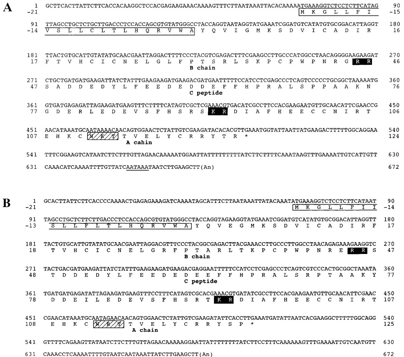
Fig. 2. Nucleotide and deduced amino acid sequences of cDNAs encoding Pos-AGH ( A ) and Pod-AGH ( B ) precursors. Amino acid numbering is commenced at the N-terminal residue of each propeptide of the Pos- and Pod-AGHs. Open and filled boxes indicate the signal peptide and a putative dibasic cleavage site, respectively. Shaded boxes indicate putative N-linked glycosylation motifs. Each polyadenylation signal sequence is underlined. The nucleotide sequences of the cDNAs encoding Pos- and Pod-AGHs have been deposited in the DDBJ/EMBL/GenBank databases (accession nos. AB089810 and AB089811, respectively).
