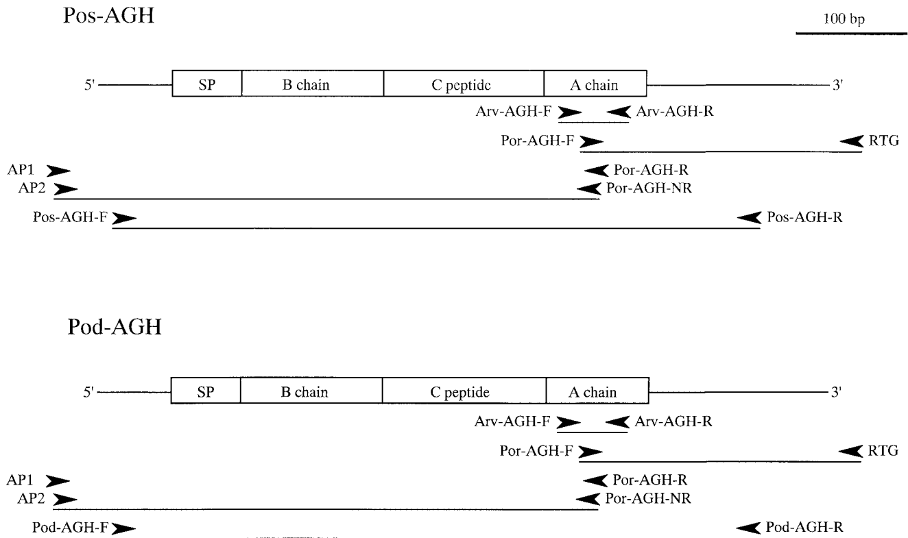
Fig. 1. Schematic representation of the structures of cDNAs encoding Porcellio scaber AGH (Pos-AGH) and P. dilatatus AGH (Pod-AGH), and the locations of oligonucleotide primers. Arrowheads represent the primers, and lines under the arrowheads indicate the cDNA fragments which were amplified. Boxes represent the open reading frame. Thin lines indicate the 5'- and 3'-untranslated regions. SP is the abbreviation for signal peptide.
