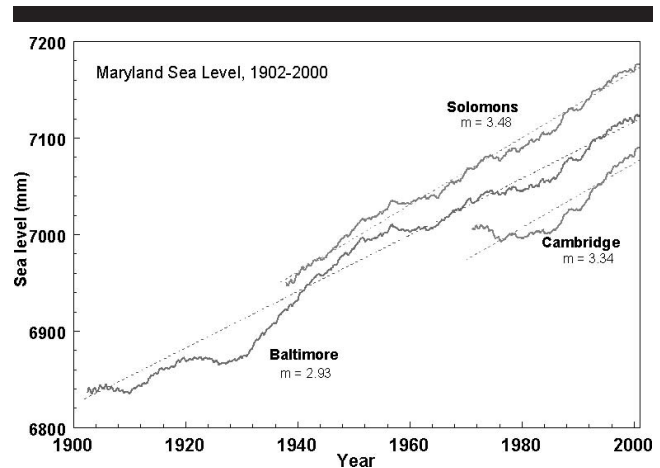
Figure 2. Maryland sea level, 1902–2000. Three tidal gauge records of monthly sea level. Data have been smoothed with a 12-month moving boxcar filter. Numbers below curves are linear fit trends in mm per year.
