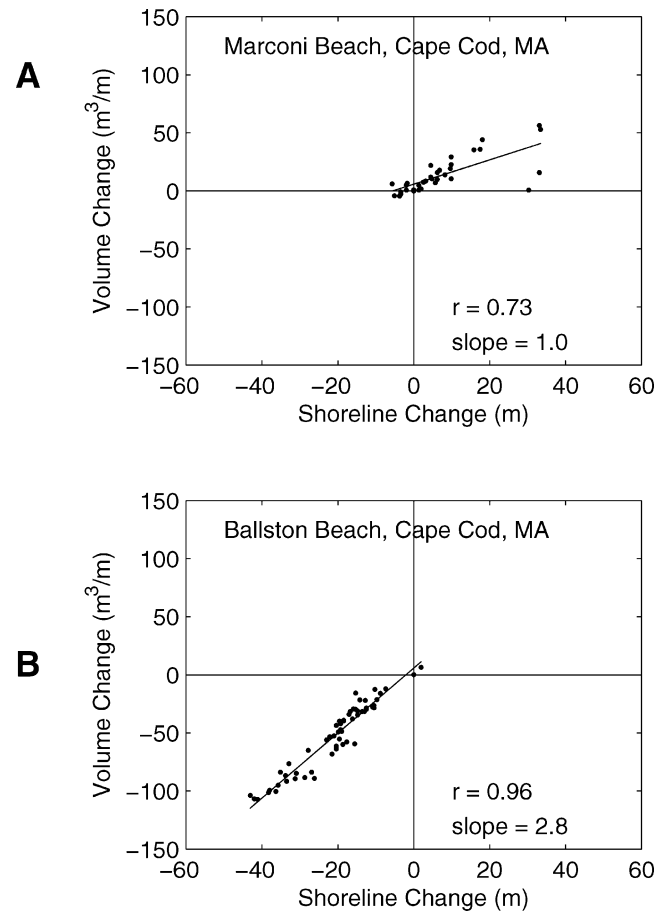
Figure 6. Subaerial volume change vs. shoreline change data from (A) Figure 5A, Marconi Beach, and (B) Figure 5B, Ballston Beach. Also shown is the best fit line through the data and its associated correlation coefficient and slope.
