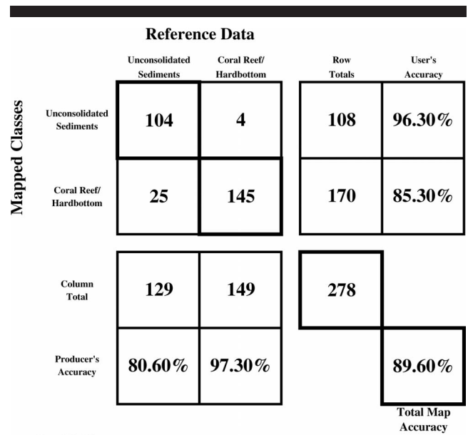
Figure 7. Confusion matrix for two generalized mapped classes: unconsolidated sediment and coral reef–hard bottom.
