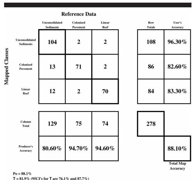
Figure 8. Confusion matrix for three generalized mapped classes: unconsolidated sediments, colonized pavement, and linear reef.
