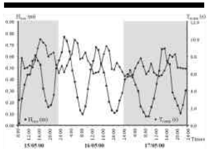
Figure 2. Offshore wave conditions during the field experiments measured at the position marked as RUNTI in Figure 1a.
