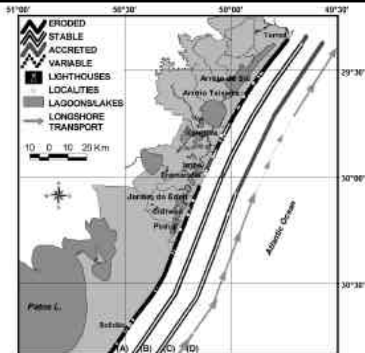
Figure 4. Shoreline changes in the northern Rio Grande do Sul littoral based on: (A) shoreline variations between 1975-2000 (ESTEVEES et al. , 2001), (B) concentration of wave energy due to short-term storm events (CALLIARI et al. , 2000), and (C) concentration of wave energy due to large-scale coastal topography (DILLENBURG et al. , 2000). Arrows show direction of littoral drift, and variations of longshore transport rates (as estimated by ALMEIDA et al. , 2001) are indicated by changes in arrows width.
