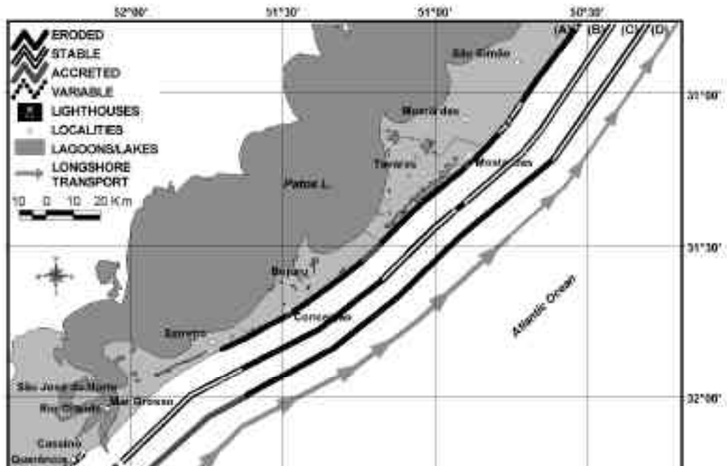
Figure 3. Shoreline changes in the central RS littoral based on: (A) shoreline variations between 1975-2000 (ESTEVEES et al. , 2001), (B) concentration of wave energy due to short-term storm events (CALLIARI et al. , 2000), and (C) concentration of wave energy due to large-scale coastal topography (DILLENBURG et al. , 2000). Arrows show direction of littoral drift, and variations of longshore transport rates (as estimated by ALMEIDA et al. , 2001) are indicated by changes in arrows width.
