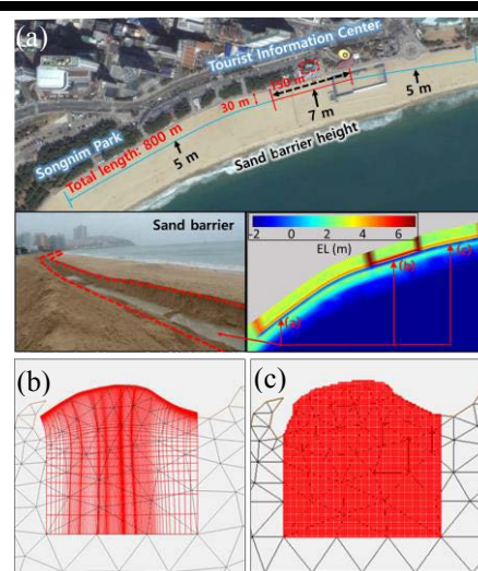
Figure 1. (a) Sand barrier specifications, (b) orthogonal curvilinear grid with minimum size of 5 m for simulation of barrier breaching, and (c) rectilinear grid for real-time forecasting with grid size of 30 m.
