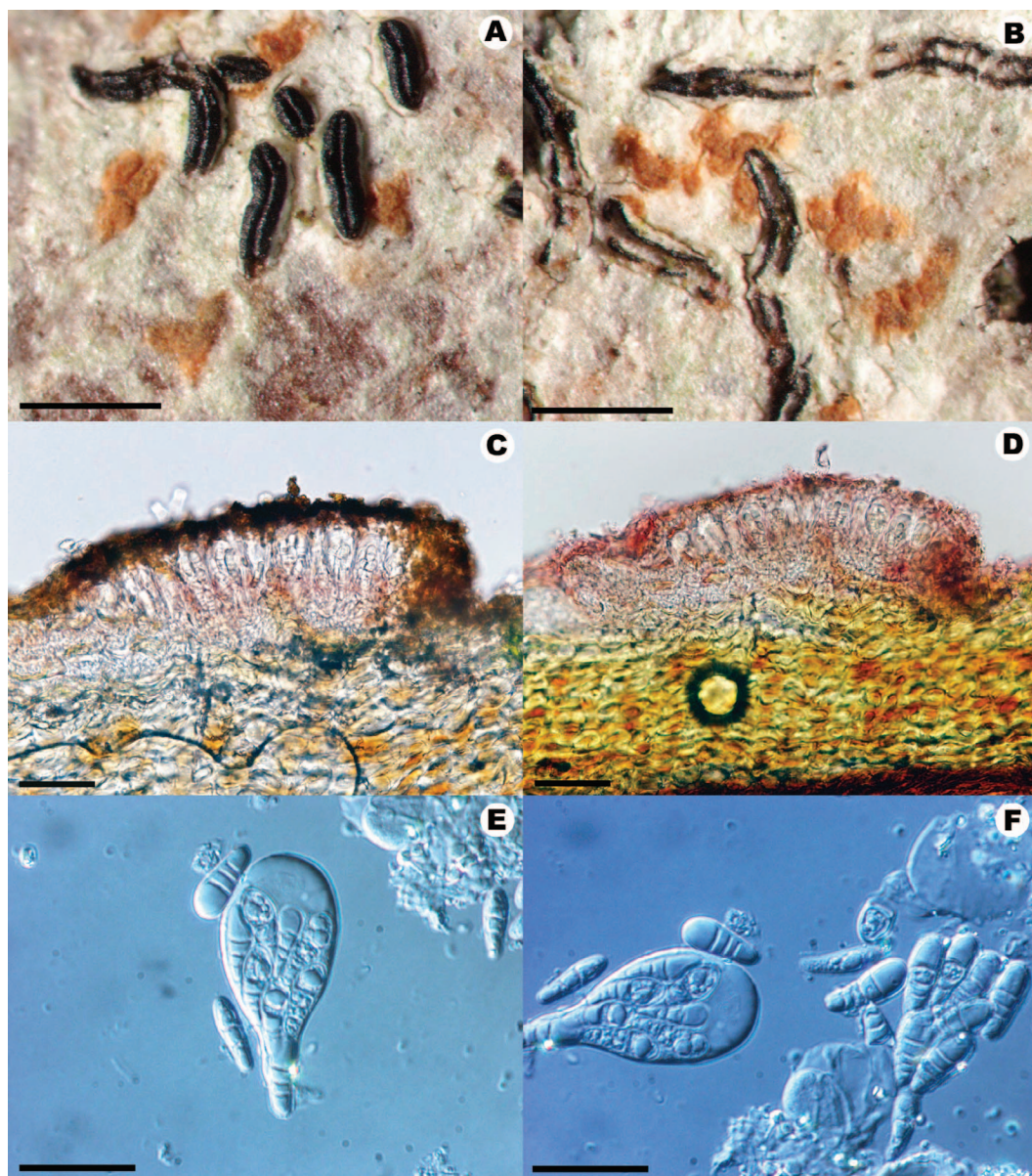
Figure 14. Arthonia hodesii (all from the holotype). A and B. Detail of fruiting bodies and infection occurring on thallus of Graphis lineola . C. Transverse section of ascus in water. D. Transverse section of ascus in K illustrating reaction of pigments. E and F. Ascus and ascospores in water. Scale bars = 500 \mu m in A and B, 50 \mu m in C and D, and 20 \mu m in E and F.
