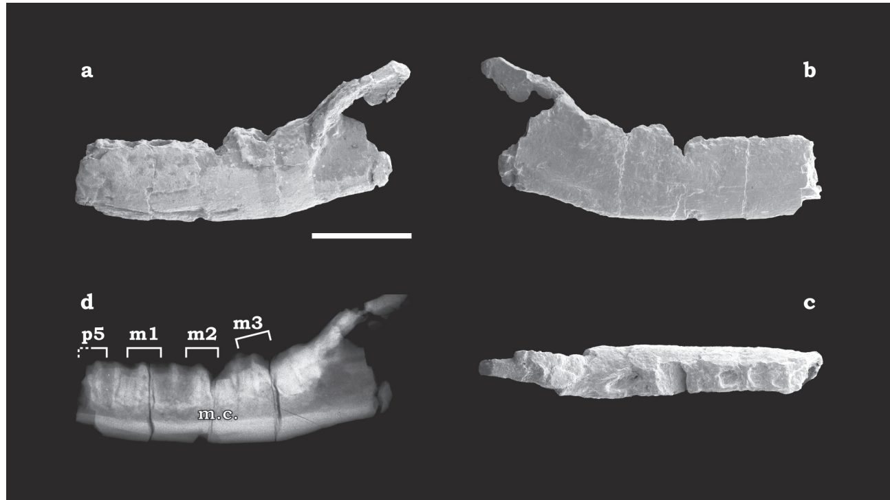
Figure 2. A fragment of eutherian left mandible (MDM 725). Scale bar is 5 mm. a , SEM photograph of MDM 725 (resin cast) in labial view; b , same in lingual view; c , same in occlusal view; d , SOFTEX photograph of MDM 725, p5 to m3 indicate alveolus for each tooth; m.c., mandibular canal.
