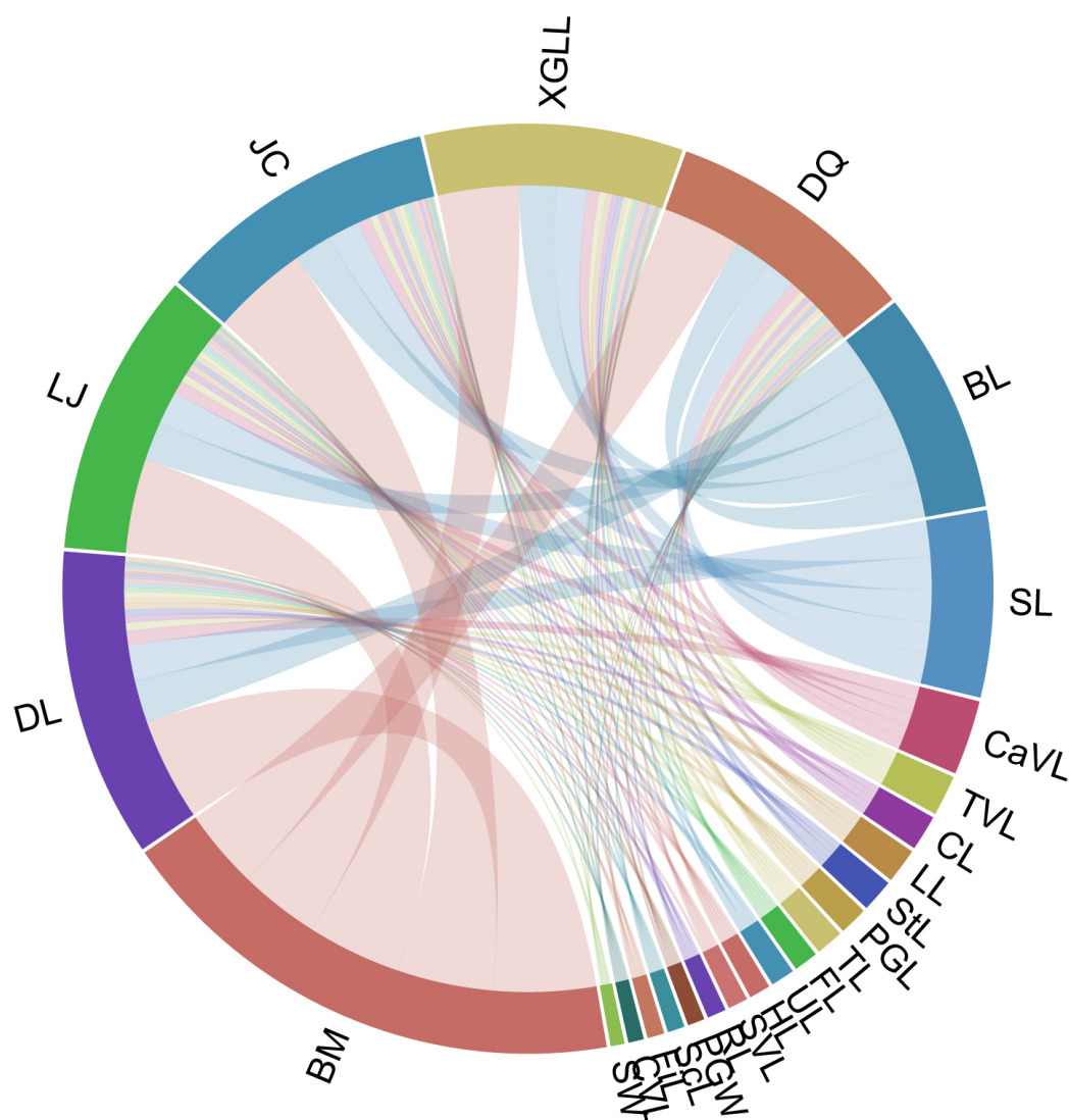
Fig. 1. Chord diagram of body mass, body length and bone length.
