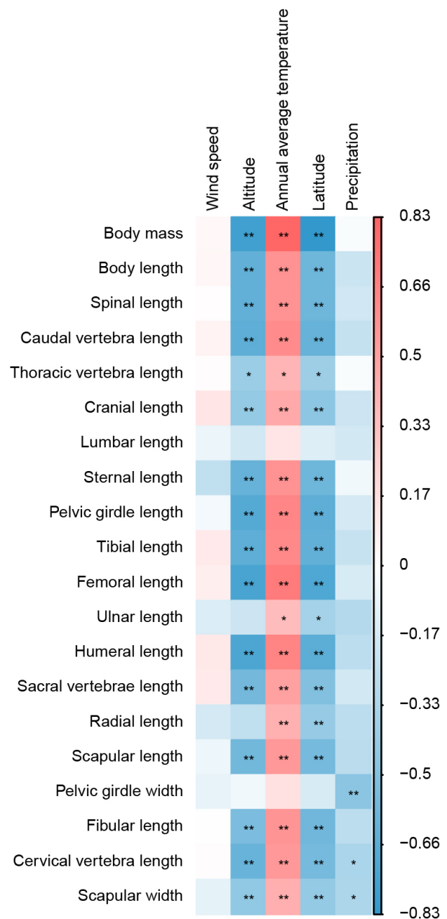
Fig. 6. Correlation analysis between body mass, body length, bone length and climate (* P < 0.05 , ** P < 0.01 ).
