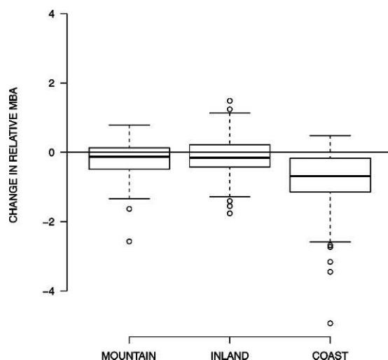
Figure 3. Change in relative herbivore pressure from 1949 to 1999 for all large herbivores in Norway in the mountain, inland and coastal regions. Herbivore pressure is based on metabolic biomass/km 2 unimproved land ( MBA_{total} ) each year. Note that the y-axis show ln-transformed values.
