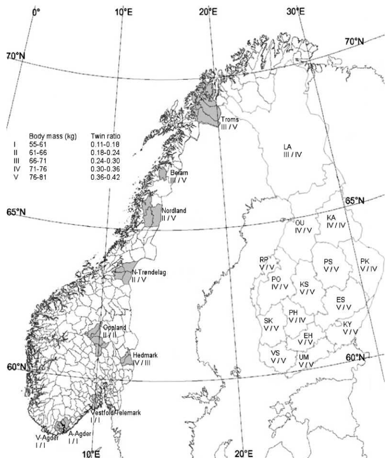
Figure 1. Our study areas in Norway (Vest-Agder, Aust-Agder, Vestfold/Telemark, Hedmark, Oppland, Nord-Trøndelag, Nordland, Beifarn and Troms) and Finland (EH = Etelä-Häme, ES = Etelä-Savo, KA = Kainuu, KS = Keski-Suomi, KY = Kymi, LA = Lappi, PH = Pohjois-Häme, PK = Pohjois-Karjala, PO = Pohjanmaa, PS = Pohjois-Savo, RP = Ruotsinkielinen Pohjanmaa, SK = Satakunta, VS = Varsinais-Suomi and UM = Uusimaa). The numerals I-V indicate the category of mean body mass of female calves and the twinning rate in the region, category I being the lowest and V the highest values, respectively.
