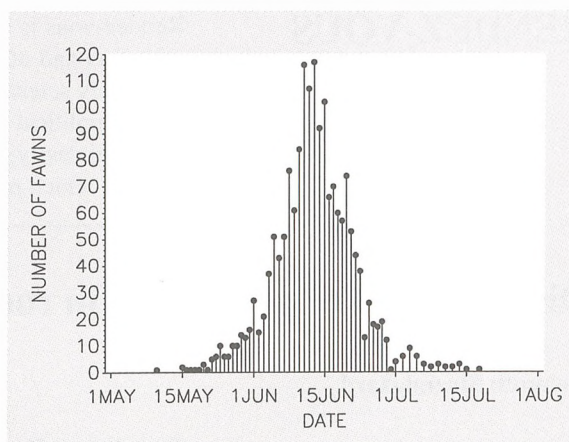
Figure 1. Extend of the fawning period in the Borris area, based on 1,692 newborn fawns, ear-tagged during 1956-1980. Eighty per cent of the births were given within 19 days.
