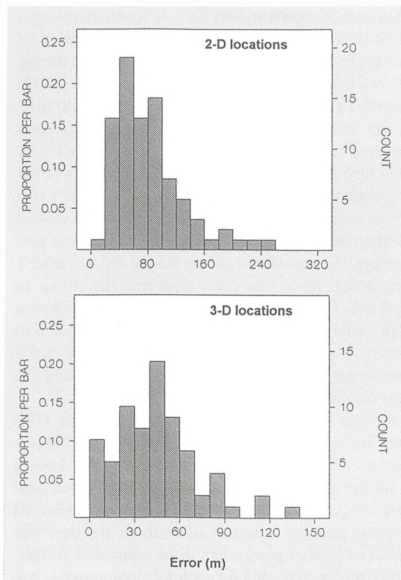
Figure 1. Frequency distribution of GPS locational error in 2-D and 3-D mode.
