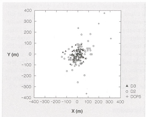
Figure 2. Spatial distribution of GPS locational error in relation to true position. D3 = 3-D locations, D2 = 2-D locations, and DOP5 = 2-D and 3-D locations with DOP > 5 .
