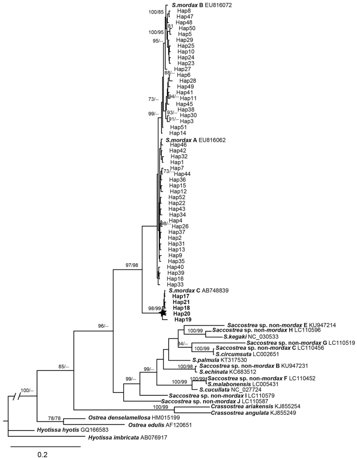
Figure 3. Bayesian phylogenetic tree of Saccostrea oysters based on partial cytochrome oxidase I DNA sequences. Numbers on nodes are posterior probability/bootstrap values (≥70).
