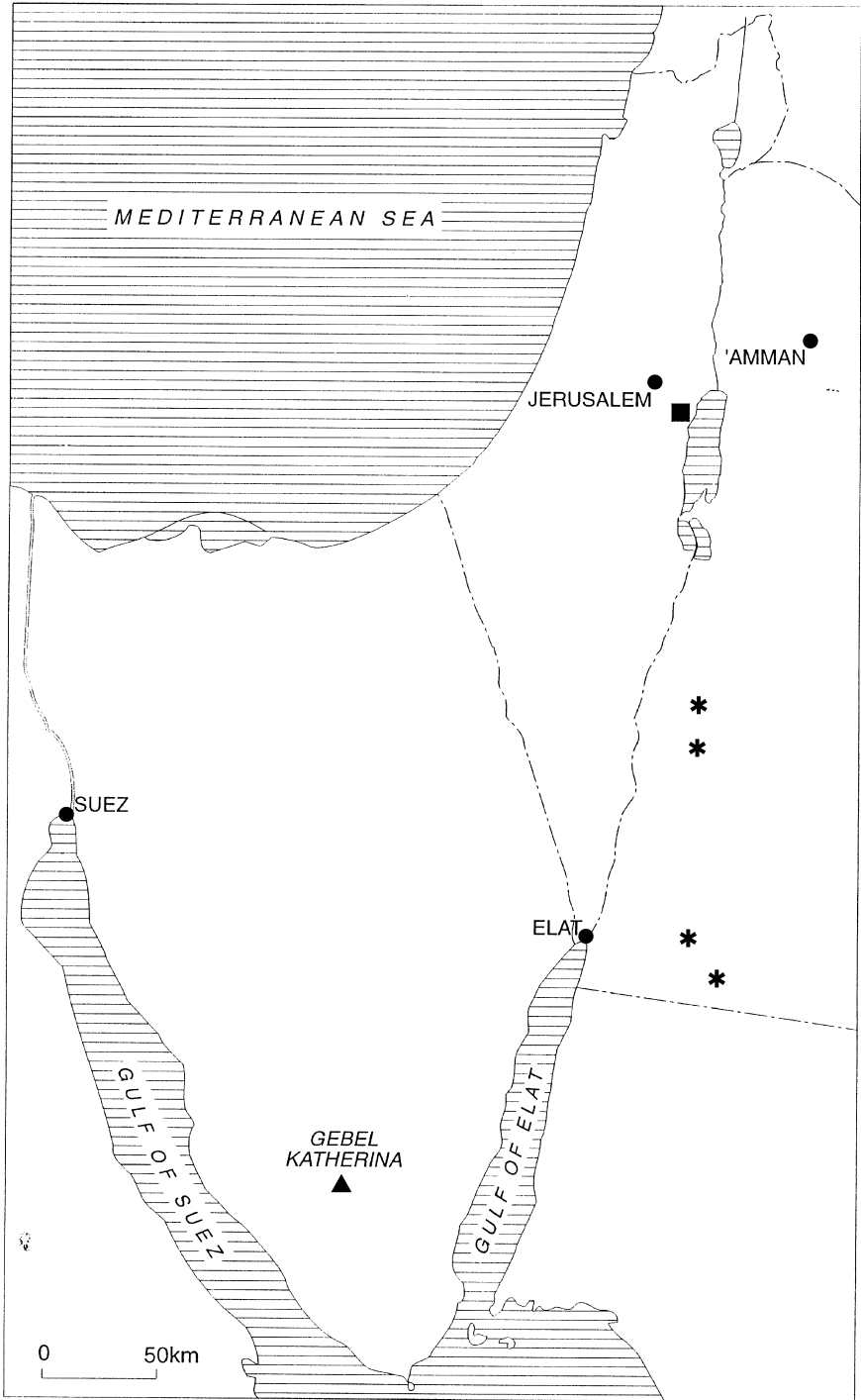
Fig. 2. Distribution of Satureja sect. Zatarioideae in Israel and Jordan – S. thymbriifolia ■, S. nabateorum *.
