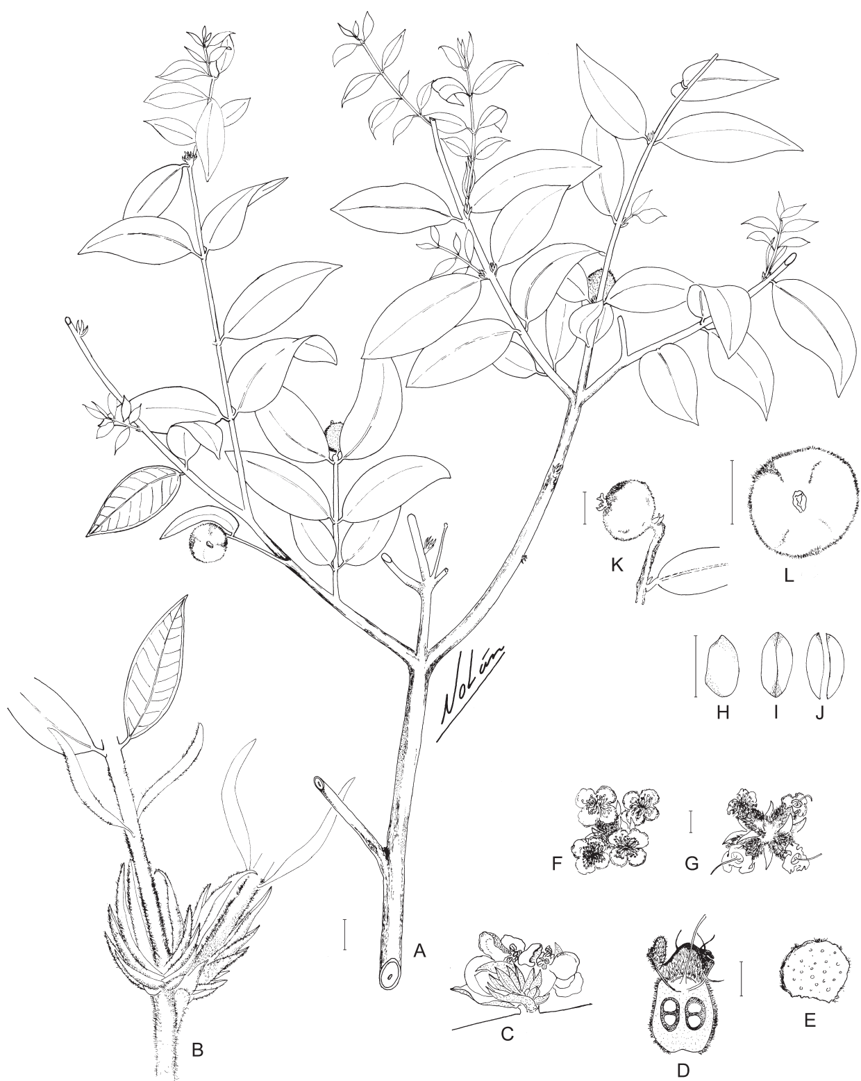
Fig. 1. Plinia arenicola – A: leafy branch with fruits; B: bud scales at the base of young branches; C: flower glomerule with surrounding involucral bracts; D: ovary in longissection, crowned by hypanthium and calyx remains; E: petal; F-G: group of 4 flowers, during and after anthesis; H: seed; I: embryo; J: embryo, with the cotyledon separated; K: fruiting twig; L: fruit in frontal view, with calyx scar. – Scale bars: A-C 10 mm, D-E 1 mm, F-G, K-L 5 mm, H-J 7 mm. Drawings by Nolán Iglesias.
