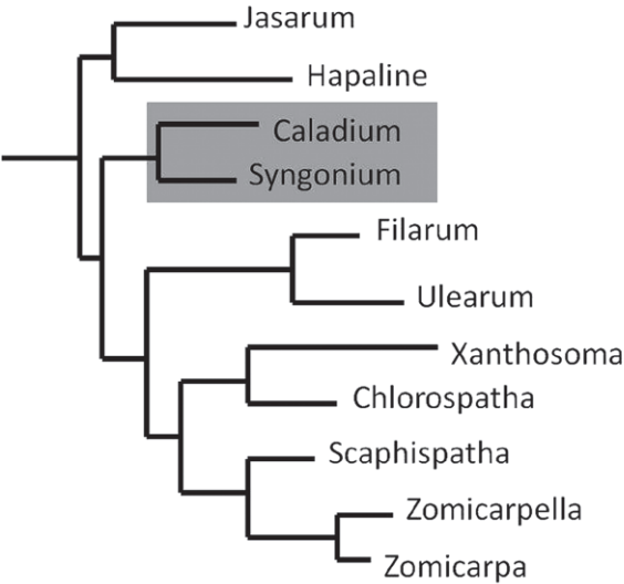
Fig. 25. Phylogenetic position of the tribe Caladieae (shaded grey) revealed by Cusimano & al. (2011) in their molecular phylogeny of the Araceae .
