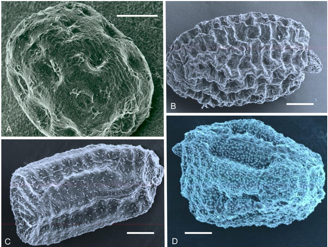
Fig. 3. SEM photographs of Linderniaceae seeds – A: Torenia crustacea ; B: Linderniella cerastioides ; C: Lindernia rotundifolia ; D: Crepidorhapon microcarpaeoides . – Scale bar 100 µm. – Photographs by E. Fischer.
