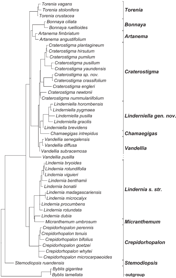
Fig. 5. Phylogram from Bayesian Inference of phylogeny with branch lengths giving the relative substitution rates using the GTR+G+I model. Taxa are named according to the taxonomic treatment suggested in this study.
