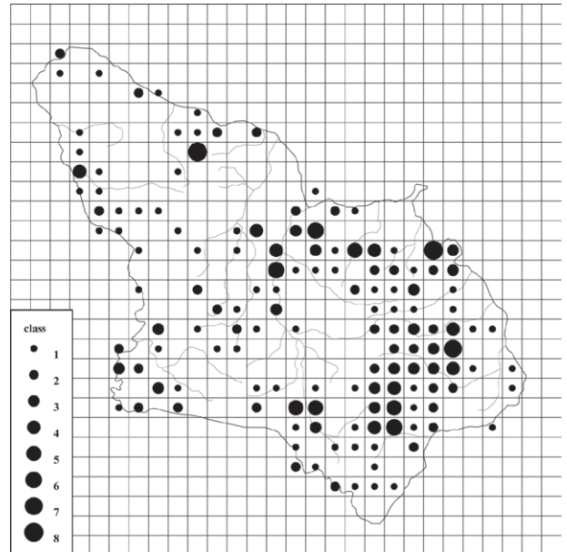
Fig. 5. Concentration map of thermophilous species of trees and shrubs. Labelling as in Fig. 3.
